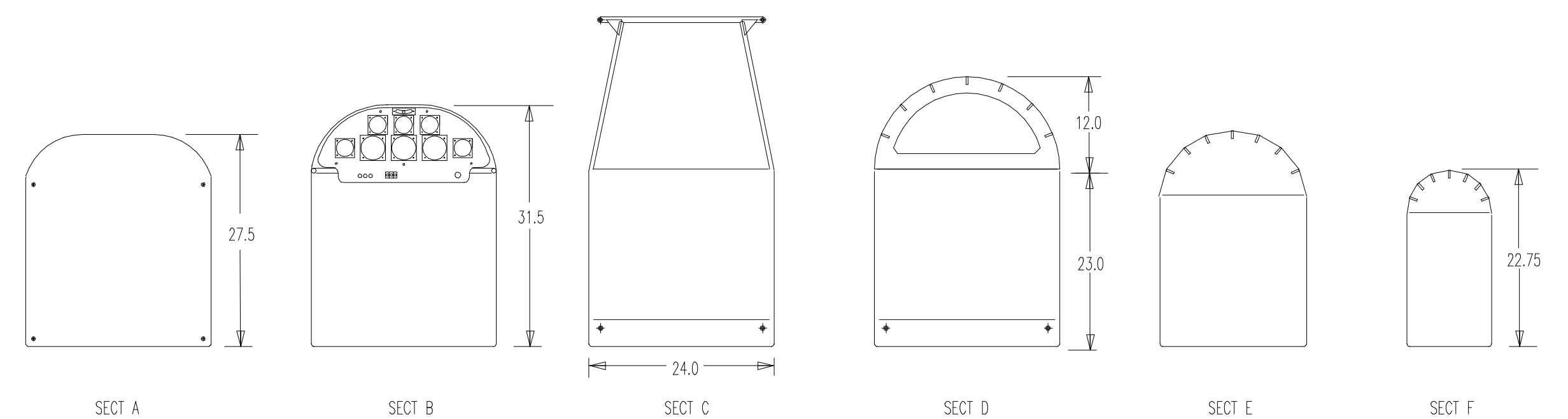
FUSELAGE SECTIONS
