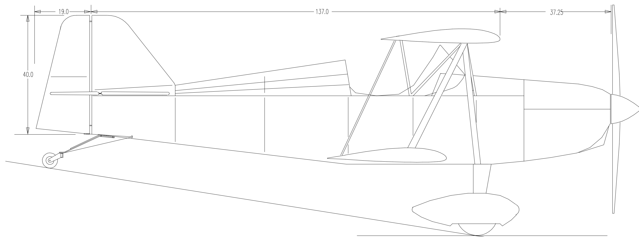
RIGHT SIDE VIEW
