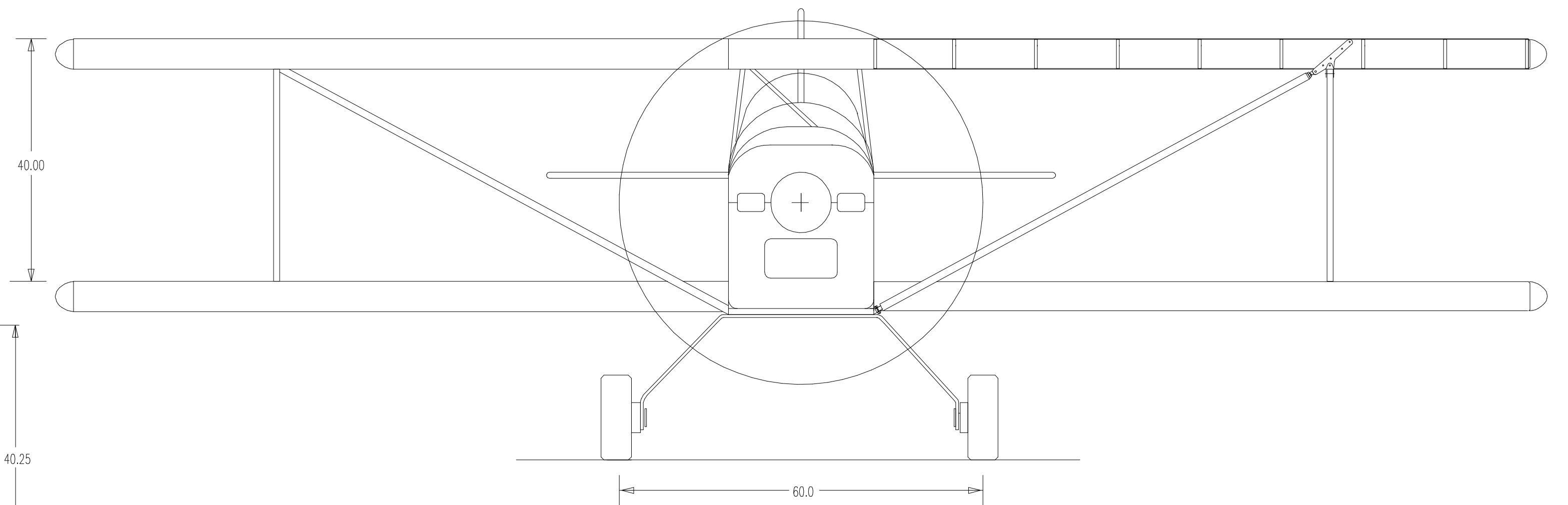
FRONT VIEW
