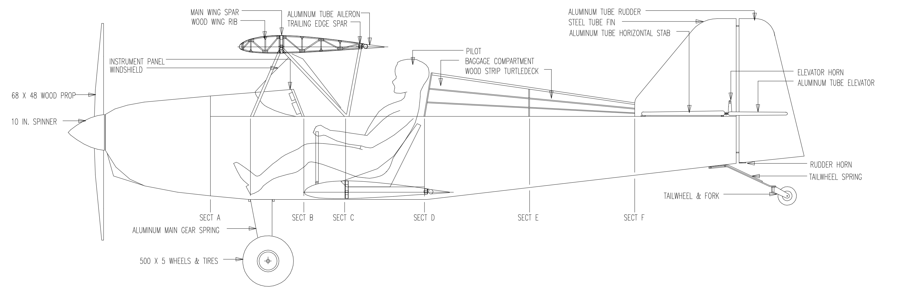
LEFT SIDE CUTAWAY VIEW
